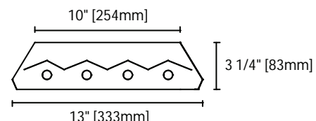
HB 4 Lamp Cross Section View
