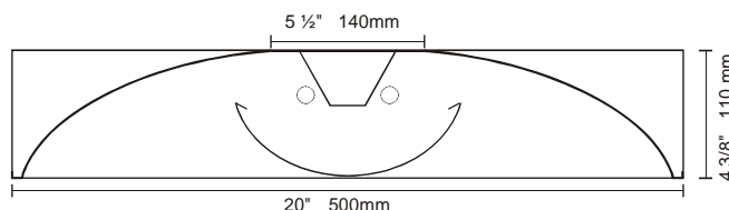
TBBK-P 2060/2048 Cross Section
